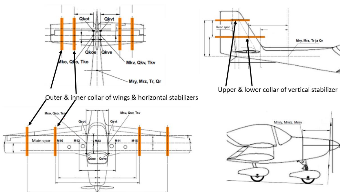
Figure 1: An overview of the on-aircraft ground calibrations. External vectorial loads applied via collars on each component.
